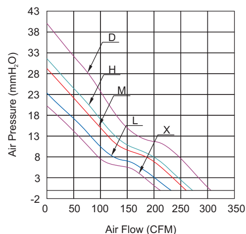
Performance Curves
